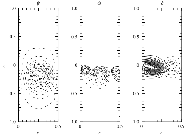
FIGURE 8. Axisymmetric perturbations of the streamfunction \hat{\psi} , vorticity \hat{\omega} and the concentration \hat{c} associated with the largest eigenvalue for R=4 , Ra=10^6 at a characteristic interface thickness of \delta=0.1 .
