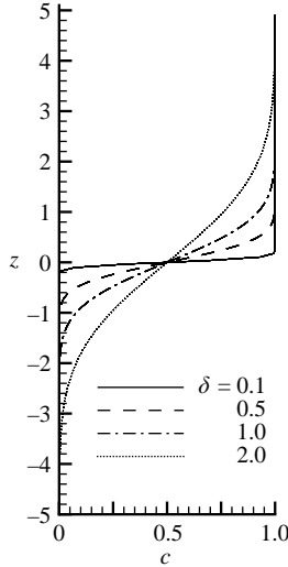
FIGURE 3. Base concentration profile \bar{c}(z) for selected values of the interfacial thickness parameter \delta .
